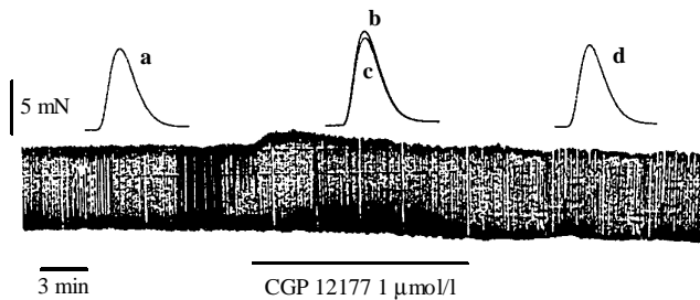
Fig. 4. Time course of the effect of CGP 12177 on contraction force of human atrial trabeculae. The upper traces show contraction at baseline ( a and d ), after 5-min ( b ) and 15-min ( c ) perfusion with 1- \mu\text{mol/l} CGP 12177. In the lower part of the figure the kinetics of contraction force is shown at low recording rate.
