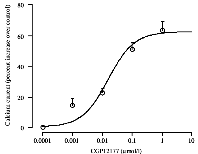
Fig. 2. Concentration-response curve for the stimulating effect of CGP 12177 on L-type Ca^{2+} current in human atrial cells. EC_{50} and E_{\text{max}} values for the effect of CGP 12177 on I_{Ca} were 0.016 \pm 0.007 \mu\text{mol/l} and 61.7 \pm 5.8 percent ( n=14 ) respectively. The open circles show the mean and the vertical lines the s.e.m. The dependence of I_{Ca} upon CGP 12177 was described well enough by the equation of Michaelis (the continuous line). The data are presented as percentage of the control values.
