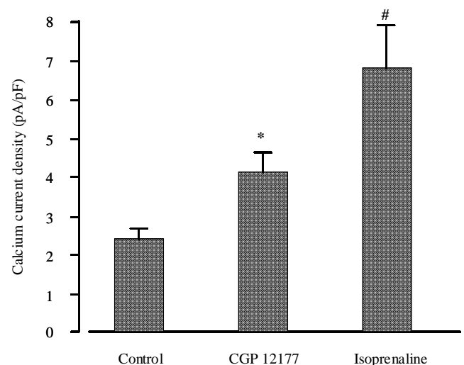
Fig. 3. Effects of 1- \mu\text{mol/l} CGP 12177 and 1- \text{mmol/l} isoprenaline on L-type Ca^{2+} current density ( n=5 ). * indicates significant difference as compared with control ( p < 0.05 ), # - as compared with CGP 12177 ( p < 0.05 ).
