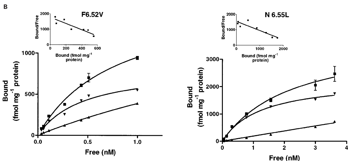
Figure 4 Saturation analysis of [ 3 H]-GR113808 binding to COS-7 cells transfected with wild-type or mutant human h5-HT 4(a) receptors. Non-specific binding was determined with 10 \mu\text{M} ML10375. Experiments were performed in triplicate using a range of nine concentrations of radioligand.
