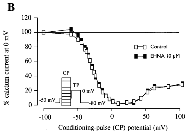
Figure 2. Voltage-dependence of the stimulatory effect of EHNA on basal I_{Ca} in a human atrial myocyte. Current-voltage relationship ( A ) and inactivation curve of I_{Ca} ( B ) in control condition ( open rectangles ) and in the presence of 10\ \mu\text{M} of EHNA ( filled rectangles ). Inactivation curves were obtained using the double-pulse protocol as indicated in the inset (see also Methods).
