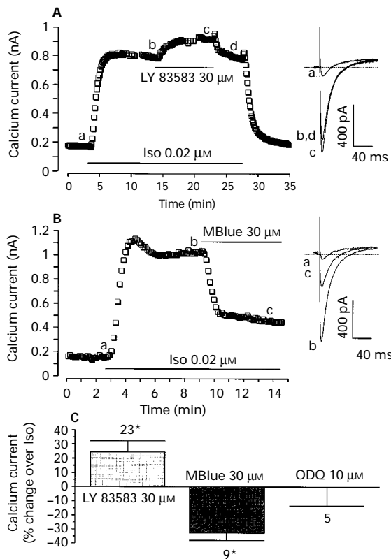
Figure 2 Effect of guanylyl cyclase inhibitors on isoprenaline (Iso)-stimulated I Ca . (A) A frog ventricular myocyte was initially superfused with control Cs + solution and dialysed with control Cs + solution. Additions of Iso (20 nM) and LY 83583 (30 μM) are indicated by the solid lines. (B) Similar experiment except that methylene blue (MBlue, 30 μM) was added in the extracellular solution. On the right, the insets show the first 125 ms of individual I Ca current traces recorded at the times indicated by the corresponding letters on the main graphs. The dotted lines indicate the zero-current level. (C) Summary of the effects of the guanylyl cyclase inhibitors on the Iso (20 and 200 nM)-stimulated I Ca . The data were normalized with respect to the amplitude of the Iso-stimulated I Ca . The columns indicate the means ± s.e. mean of the number of experiments indicated. Significant differences from the Iso level are indicated as: *P < 0.01.
