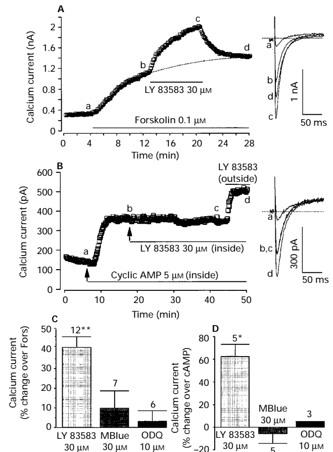
Figure 3 Effects of guanylyl cyclase inhibitors on forskolin- or cyclic AMP-stimulated I Ca . In (A) and (B) frog ventricular myocytes were initially superfused with control Cs + solution and dialysed with control Cs + solution. In (A) the cell was superfused with forskolin (0.1 μM), on the top of which LY 83583 (30 μM) was added, as indicated by the solid line. In (B) internal dialysis with 5 μM cyclic AMP was started at the first arrow and continued throughout the rest of the experiment. LY 83583 30 μM was added in the intracellular solution at the time indicated by the second arrow. Addition of LY 83583 (30 μM) in the extracellular solution was performed as indicated by the solid line. On the right, the insets show the first 125 ms of individual I Ca current traces recorded at the times indicated by the corresponding letters on the main graphs. The dotted lines indicate the zero-current level. (C) and (D). A summary of the effects of guanylyl cyclase inhibitors on I Ca previously enhanced either by forskolin (0.1 μM) in (C), or cyclic AMP (5 or 10 μM) in (D). The data were normalized with respect to the amplitude of the stimulated I Ca . The columns indicate the means ± s.e. mean of the number of experiments indicated. Significant differences from the stimulated level are indicated as: *P < 0.0, **P < 0.01.
