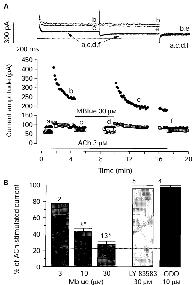
Figure 6 Effects of guanylyl cyclase inhibitors on the activation of I_{K,ACh} by acetylcholine (ACh). (A) A frog atrial myocyte was initially superfused with control K^+ solution and internally dialysed with control K^+ solution. Each symbol is the measurement of the steady-state current at -80 mV (squares), or 0 mV (circles). Applications of ACh (3 μM) in the absence or presence of methylene blue (MBlue, 30 μM) are indicated by the solid lines. (Top) Individual current traces recorded at the times indicated by the corresponding letters on the main graph. The dotted line indicates the zero-current level. (B) A summary of the effects of LY 83583, ODQ and of three concentrations of MBlue on I_{K,ACh} in the presence of 3 or 10 μM ACh. The amplitude of the end pulse current at 0 mV in the presence of MBlue plus ACh was normalized with respect to the amplitude of the current in the presence of ACh alone. In (B), the dotted line indicates the mean basal level of the steady-state current at 0 mV, in the absence of any drug. The columns indicate the means \pm s.e. mean of the number of experiments indicated. Significant differences from the ACh level are indicated as: * P < 0.01 .
