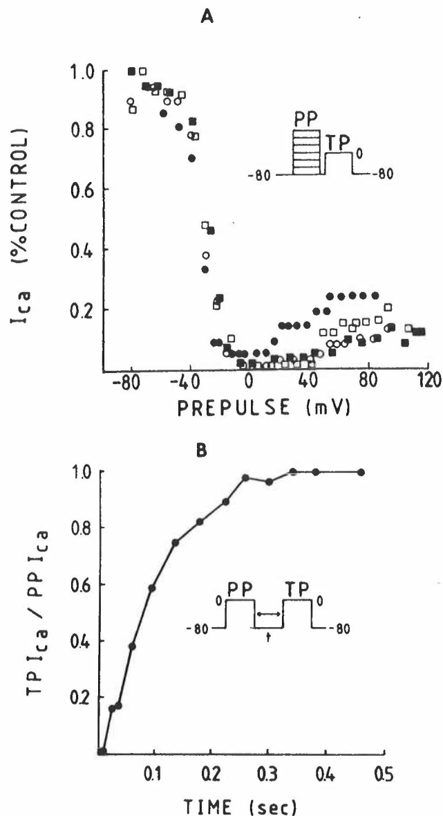
Figure 6. Inactivation and reactivation of I_{Ca} . (A) Inactivation as measured by a double pulse protocol. The amplitude of I_{Ca} elicited by a test pulse (TP) is plotted as a percentage of the I_{Ca} evoked by a step from -80 to 0 mV in the absence of a prepulse. The symbols correspond to different cells. (B) Reactivation. The ratio between the amplitude of I_{Ca} elicited by a test pulse (TP) and I_{Ca} elicited by a prepulse (PP) is plotted as a function of the interval between the pulses. The results are from a single experiment.
