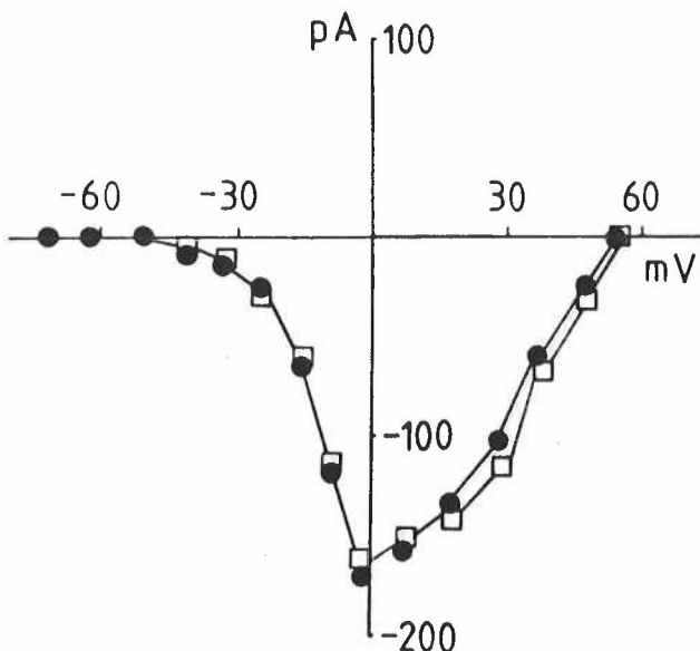
Figure 5. Net I_{\text{Ca}} of toad atrial cells. (○) Net I_{\text{Ca}} determined by subtracting I_{200} (squares in figure 4) from peak currents (filled circles in figure 4). (●) Cd-sensitive current obtained by subtracting peak current in the presence of Cd (filled circles in figure 4) from the peak currents in the absence of Cd (empty circles in figure 4).
