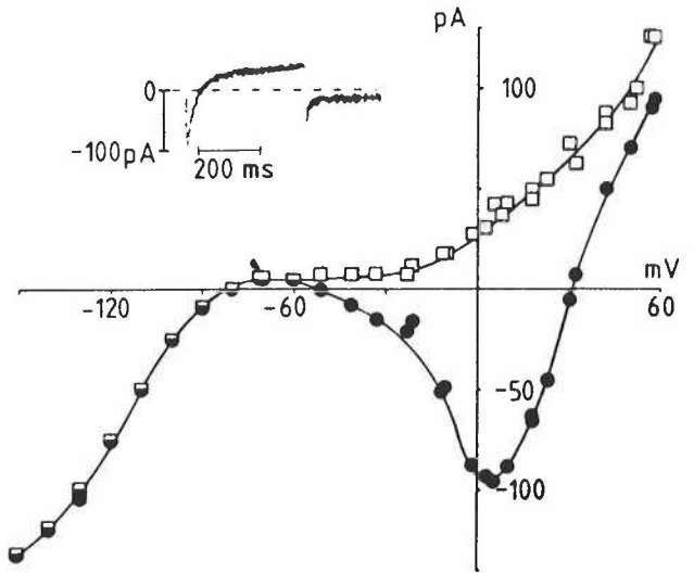
Figure 3. Current components in single cells from toad atrium. Inset: current record obtained in a cell in experimental solution # 1 with 6 \times 10^{-7} TTX, depolarized to +3 mV by a 400 ms pulse. Holding potential -80 mV. (B) Current-voltage relations obtained from peak currents ( \bullet ) and currents at the end of the pulse ( \square ) in records similar to the one shown in (A).
