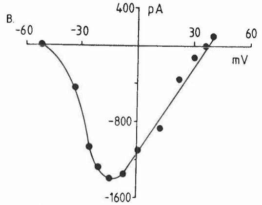
Figure 2. Sodium currents in single cells from toad atrium. (A) Records of sodium currents obtained with different depolarizations from a holding potential of -80 mV. Actual values of membrane potential are given for each record. (B) Peak current-voltage relationship obtained in the same cell. Curve fitted by eye.
