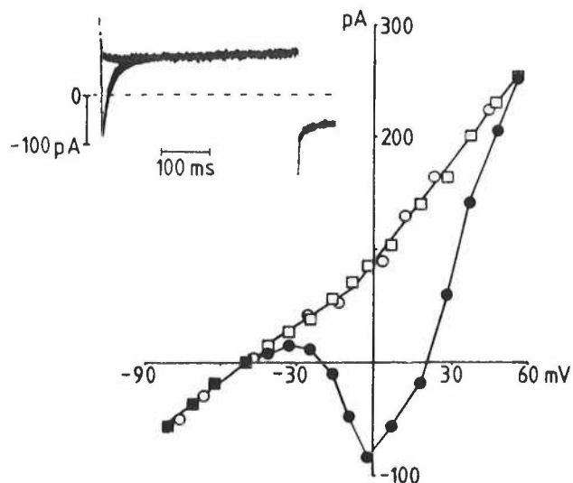
Figure 4. Measurement of I_{\text{Ca}} in single cells isolated from toad atrium. Inset: current records obtained in the presence (upper) and the absence (lower) of 0.1 mM \text{CdCl}_2 , using a depolarizing pulse of 400 ms duration which changed the membrane potential to -2 mV. B. Current voltage relationships of currents in the presence and absence of 0.1 mM \text{CdCl}_2 . Currents were elicited by 400 ms voltage steps from a holding potential of -80 mV. (●) Peak current in absence of \text{CdCl}_2 . (○) Quasi-steady state current at 200 ms ( I_{200} ) in the absence of \text{CdCl}_2 . (●) Peak currents and I_{200} in the presence of 0.1 mM \text{CdCl}_2 .
