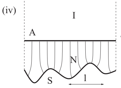
FIG. 2. Schematic representation of the nematic wet state on a rough substrate of typical l at isotropic-nematic phase coexistence.
