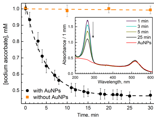
Fig. 4 Kinetic of ascorbate oxidation in the presence of 0.5 mM of \text{H}_2\text{O}_2 without (orange squares) and with AuNPs (black dots, D_{\text{AuNP}} = 20 nm, [Au] = 1 mM) in deoxygenated aqueous solution (Ar atmosphere). Inset: an example of UV-vis absorption spectra evolution of the solution containing AuNPs.
