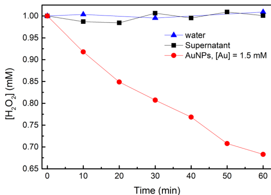
Fig. 3 Stability of \text{H}_2\text{O}_2 in absence (blue – in water, black – in supernatant solution) and presence of AuNPs [Au] = 1.5 mM (red). \text{H}_2\text{O}_2 concentration was measured by \text{TiOSO}_4 assay at pH 7. The concentration measurement is estimated to have an accuracy of ca. 6%.
