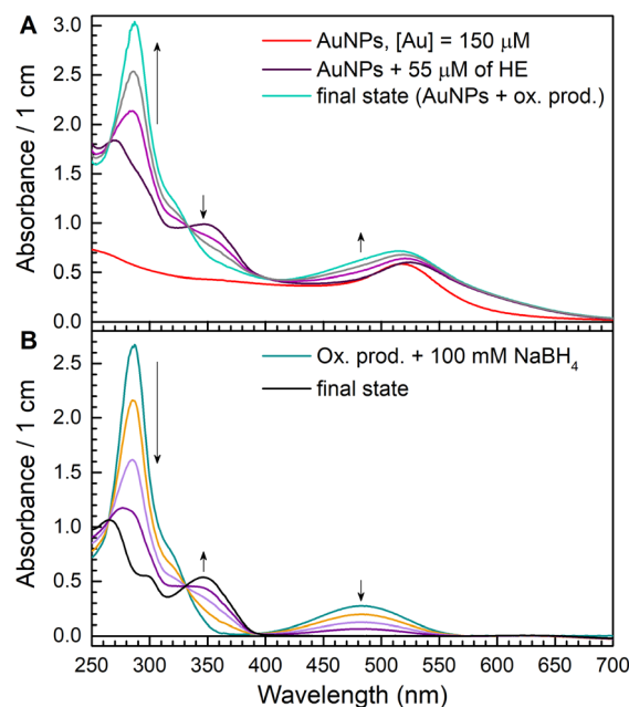
Fig. 2 Oxidation of HE (55 \mu M) by oxygen (256 \mu M, air atmosphere) in the presence of AuNPs ( [Au] = 150 \mu\text{M} ) – (A) the resulting oxidation product was purified from AuNPs by centrifugation. Reduction of the oxidation product by NaBH_4 (100 \mu M) – (B).
